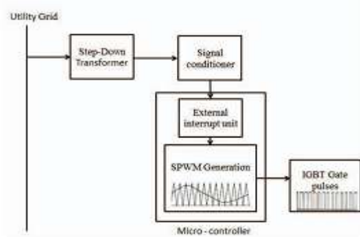
Fig.3: Frequency control system.
