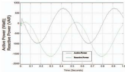
Fig. 1: Power flow due to frequency variations
