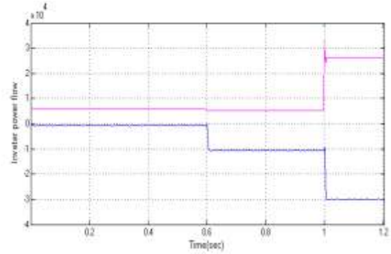
Fig 10 Automatic control of active power and DC link voltage
