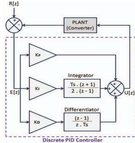
Fig. 4: PID Control System for Power Angle Control
