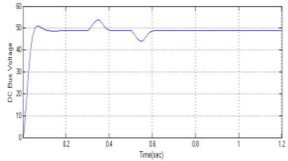
Fig 12 simulation wave form of DC link voltage
